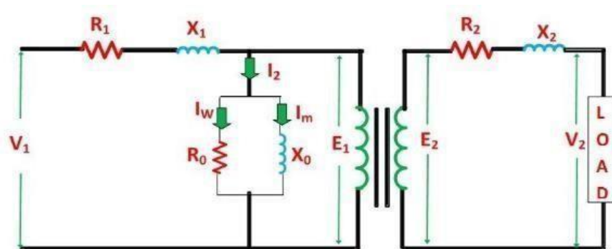
Fig: Equivalent circuit diagram of a transformer
