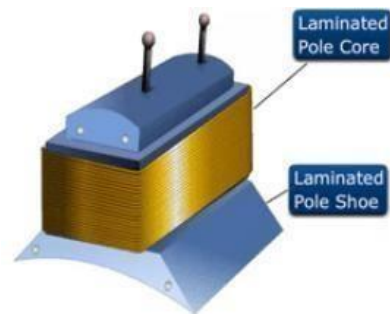
Figure 2: Pole Core and Poles Shoes representation
