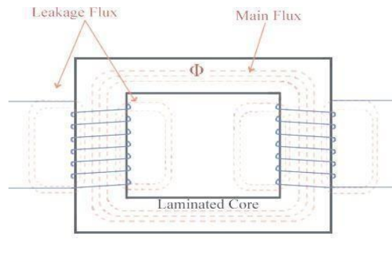
Fig: Magnetic Leakage flux
